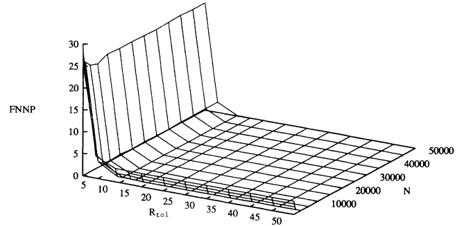
FIG. 12. Data from the two-dimensional Ikeda map in d=4 . The false-nearest-neighbor percentage is evaluated as a function of R_{\text{tol}} and the length of the data set N . d=4 is clearly a good choice for embedding this system with the use of time delay coordinates. This is consistent with the observations in Ref. [15].
